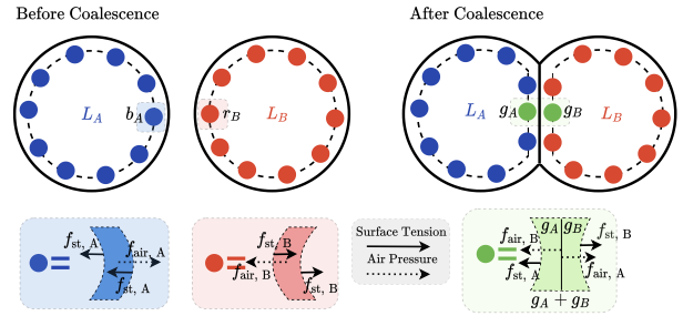
Fig. 8. The formation of a double-bubble. The top row shows the particle perspective; the bottom row depicts the control volumes with force analysis.
